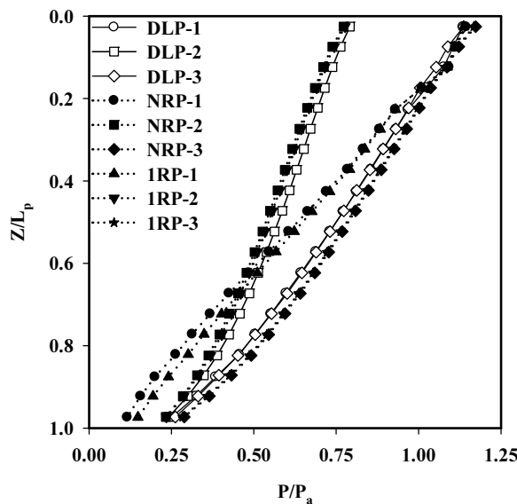
Fig. 9. Distributions of normalized axial pile forces with depth
