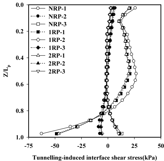
Fig. 14. Distributions of tunneling-induced interface shear stresses with depth
