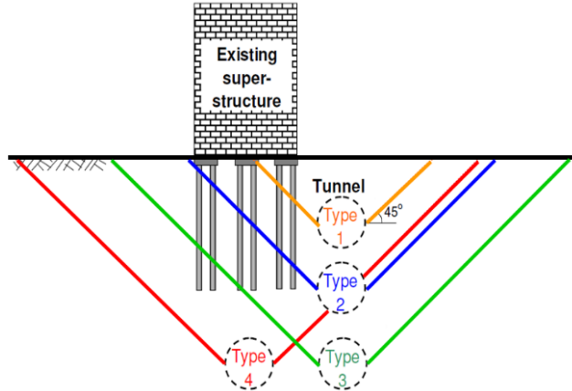
Fig. 1. Relative tunnel-pile configurations observed in practice (Pang, 2006)
